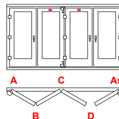
Diagrama 532 (L. marco 2580 ~ 4580mm)
