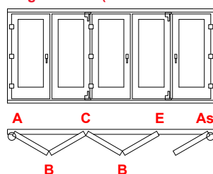
Diagrama 651 (L. marco 3200 ~ 5400mm)
