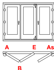
Diagrama 541 (L. marco 2640 ~ 4610mm)
