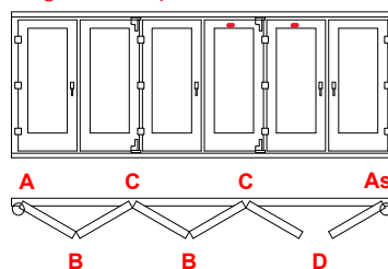
Diagrama 761 (L. marco 3700 ~ 6000mm)
