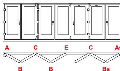
Diagrama 743 (L. marco 3700 ~ 6000mm)
