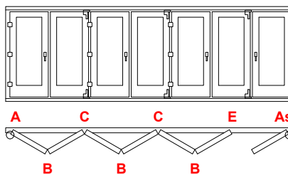
Diagrama 743 (L. marco 3700 ~ 6000mm)
