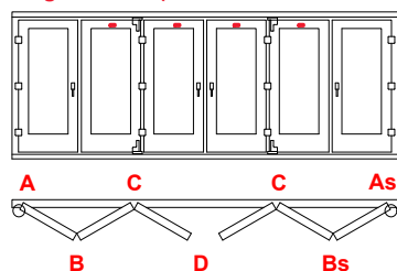
Diagrama 770 (L. marco 3700 ~ 6000mm)
